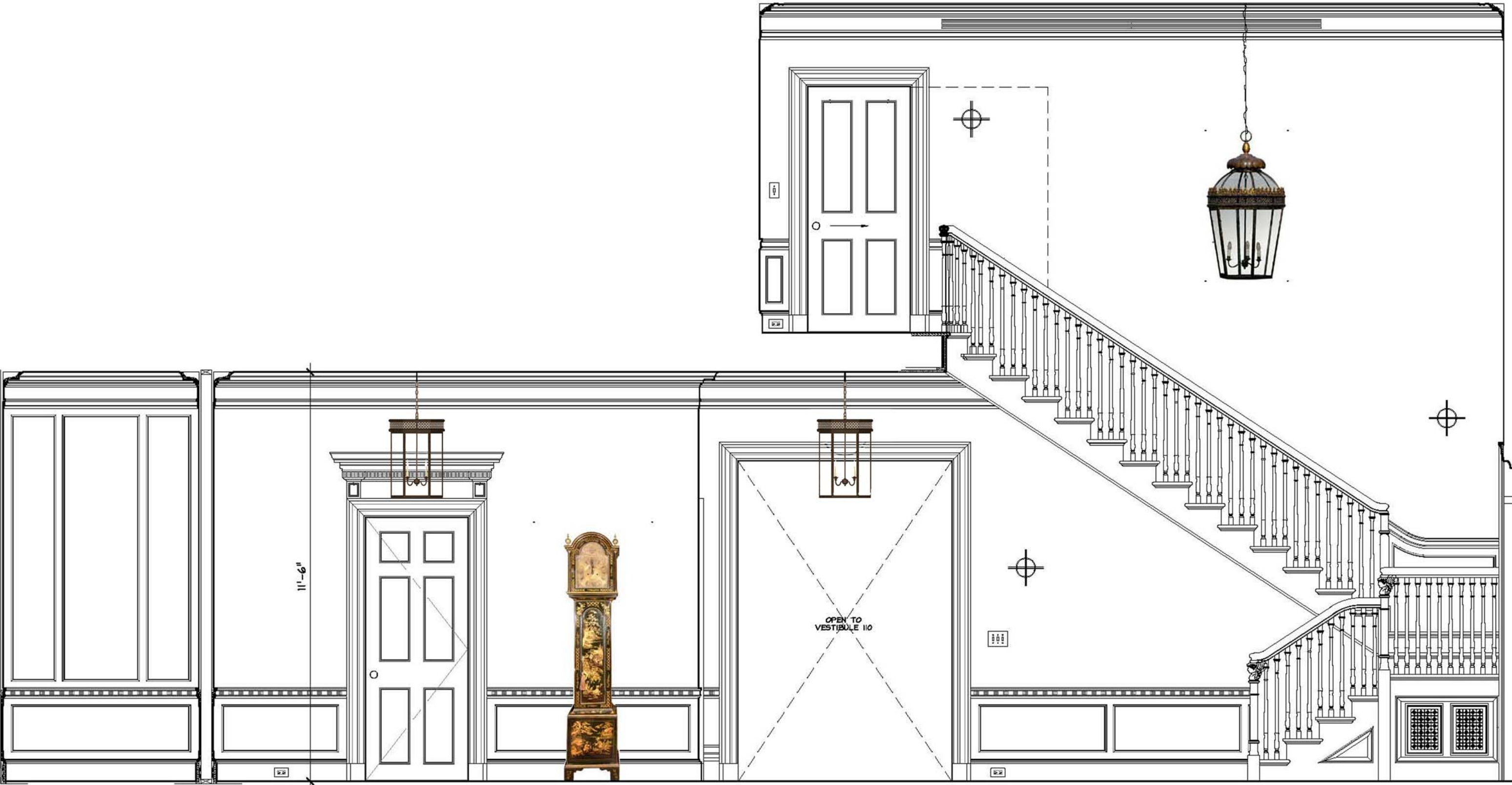
Entry Hall: West Elevation 135 Warren Street
